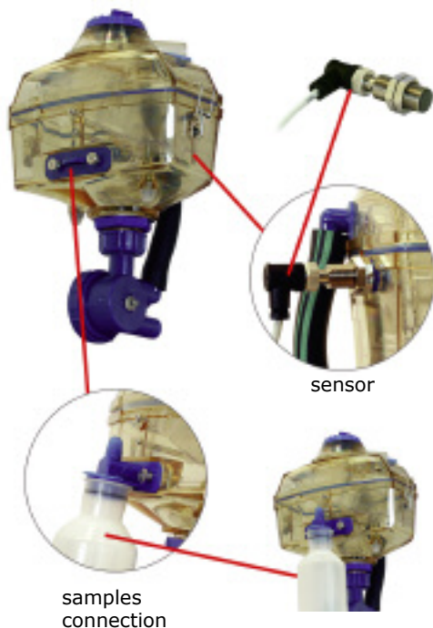
60080 Conductivity Sensor Assembly
