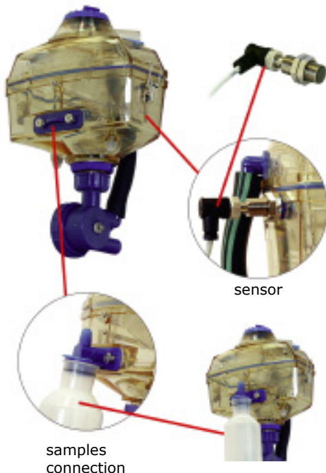
60090 Temperature and Conductivity Sensor
